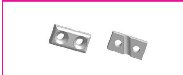
C24-Forearm_tube_enclosure
